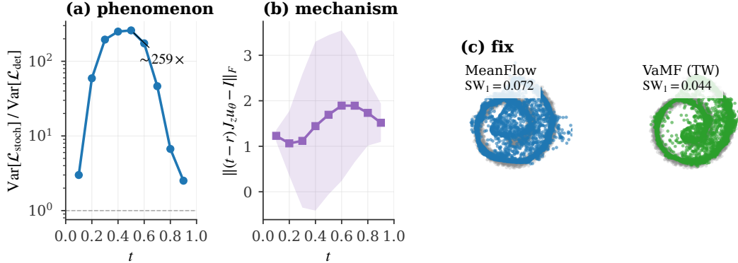
Figure 1: Variance amplification in vanilla MeanFlow and the trace-weight fix. (a) Variance ratio \text{Var}[\mathcal{L}_{\text{stoch}}]/\text{Var}[\mathcal{L}_{\text{det}}] peaks at \sim 259\times near t \approx 0.4 , in direct empirical agreement with theorem 1. (b) Frobenius norm \|(t-r)J - I\|_F peaks in the same regime, identifying the linearised flow Jacobian’s deviation from identity as the immediate source of (a). (c) The trace-weight reweighting reduces \text{SW}_1 on swiss_roll from 0.072 (MeanFlow) to 0.044 (VaMF-TW) at matched seed and step count.
