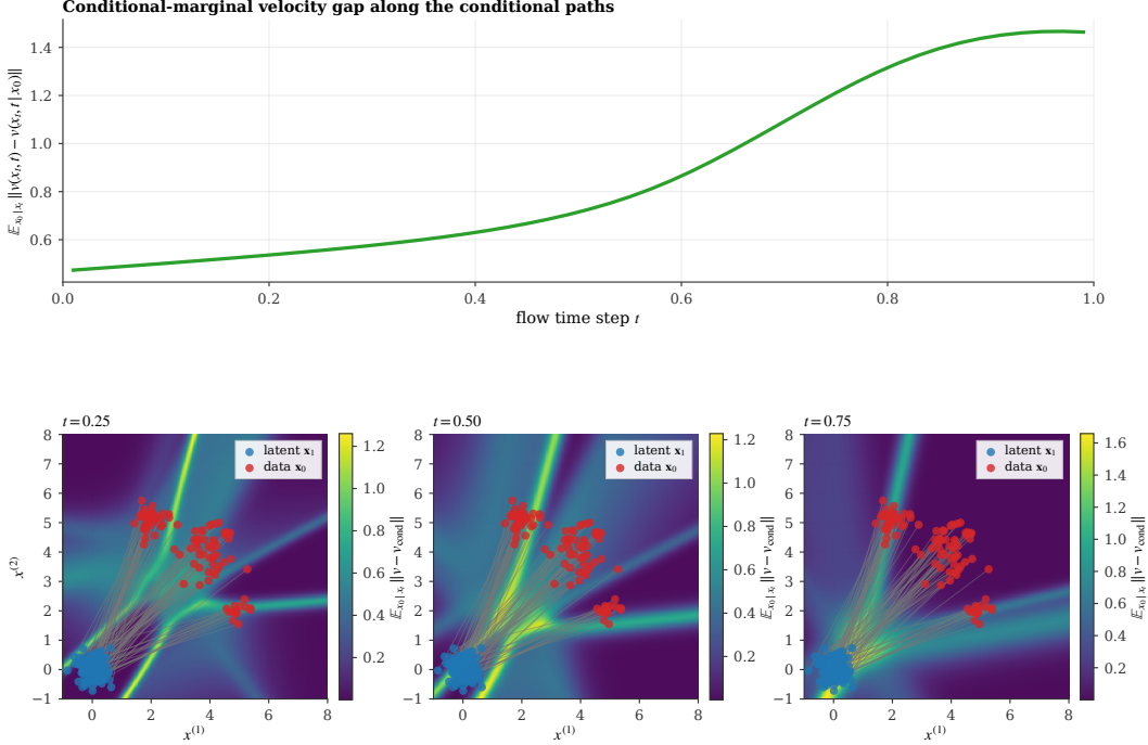
Figure 2: Conditional-marginal velocity gap on a 3-mode mixture. Top: the expected per-sample fluctuation \mathbb{E}_{x_0|x_t} \|\mathbf{v}(\mathbf{x}_t, t) - \mathbf{v}(\mathbf{x}_t, t | \mathbf{x}_0)\| , evaluated along the conditional paths, grows monotonically with t as conditional trajectories disperse, with the steepest rise where \mathbf{x}_t traverses the mode-mixing region. Bottom: the spatial heatmap of the same quantity at three timesteps confirms that the gap is heterogeneous and concentrates in the mode-mixing regions where multiple conditional paths overlap. This is the empirical realization of \Sigma_{v'} in equation 10, which the Jacobi factor \mathbf{J} amplifies into the gradient variance of theorem 1; the same regions are where the curvature gap of theorem 3 is largest, motivating the trace-weight reweighting of equation 17.
