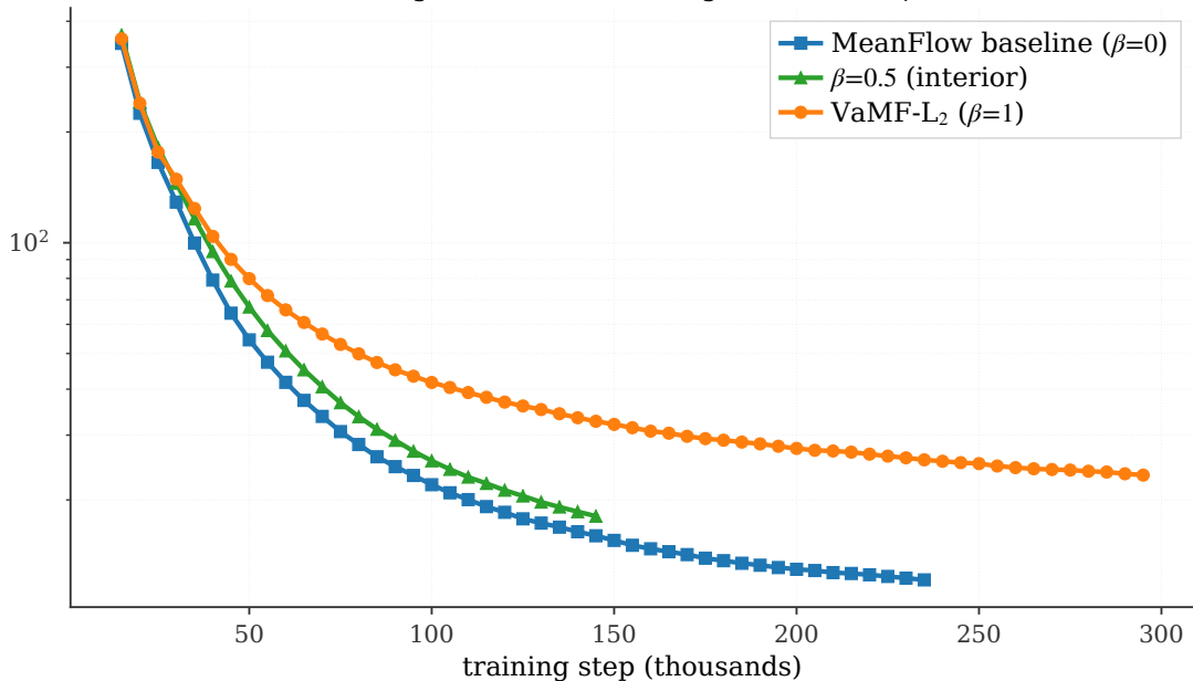
DiT-B/4 ImageNet-256 FID convergence at three \beta values
