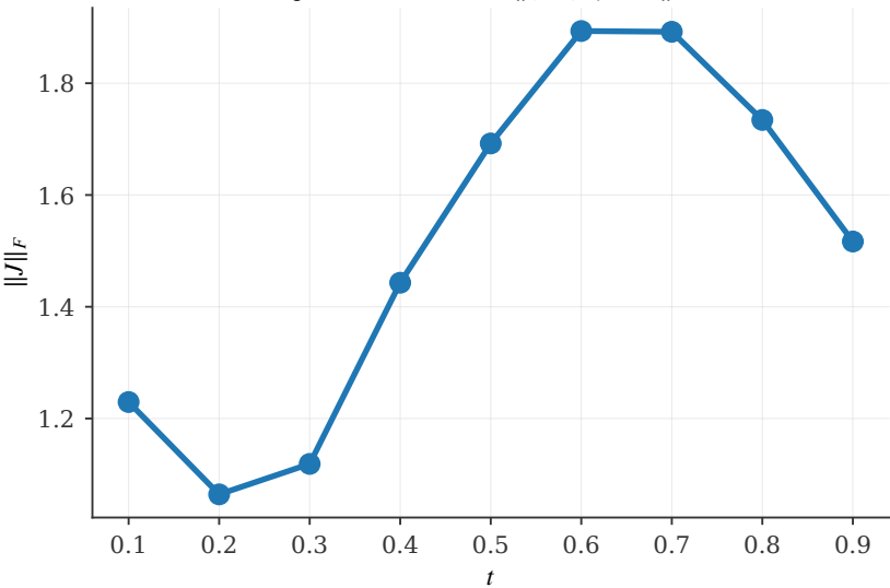
Jacobian Factor \|(t-r)\partial_z u_\theta - I\|_F
