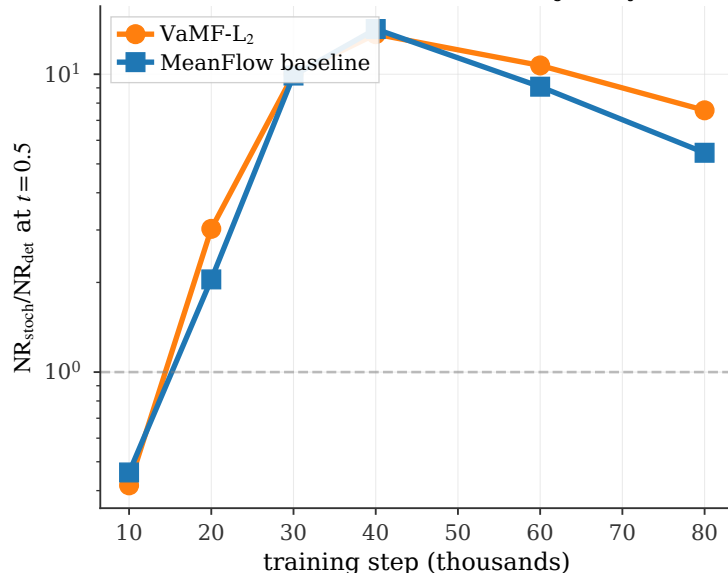
(b) Gradient-NR reduction trajectory
