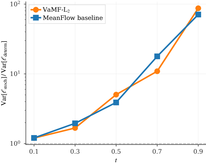
(a) Variance amplification (step 80k)
