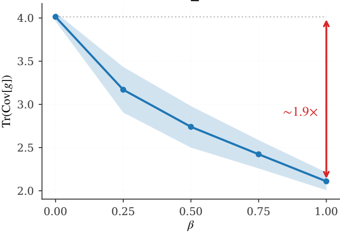
swiss_roll
