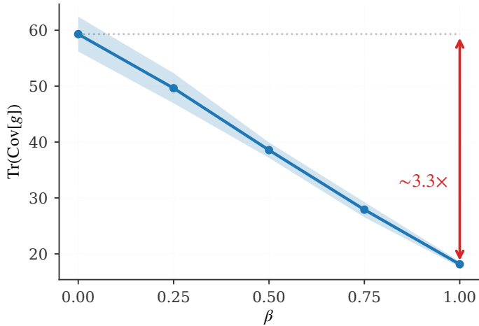
checkerboard
