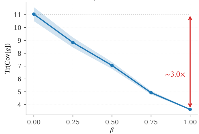
pinwheel
