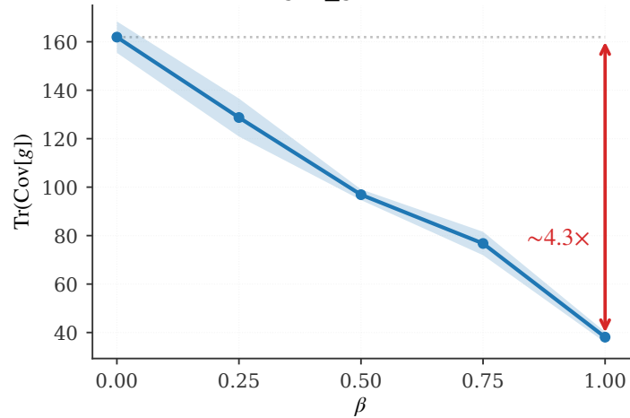
eight_gaussians
