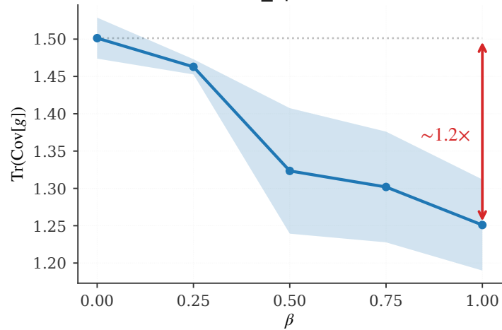
two_spirals
