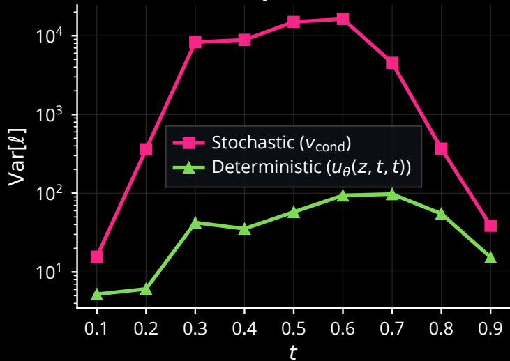
(b) Per-Sample Loss Variance
