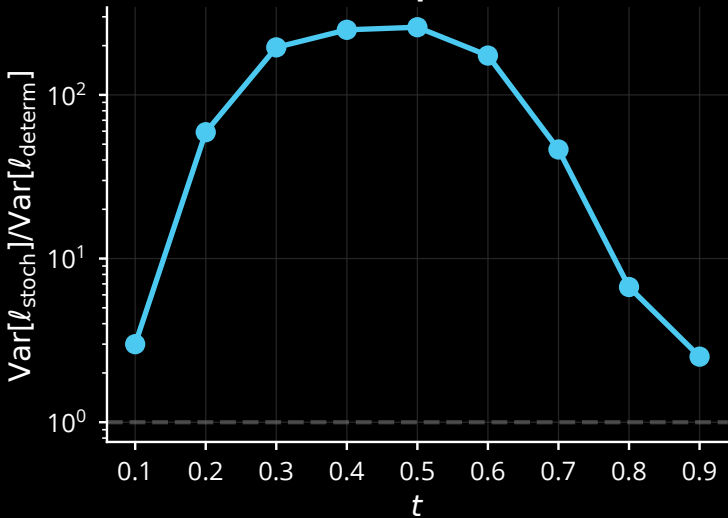
(a) Variance Amplification Ratio
