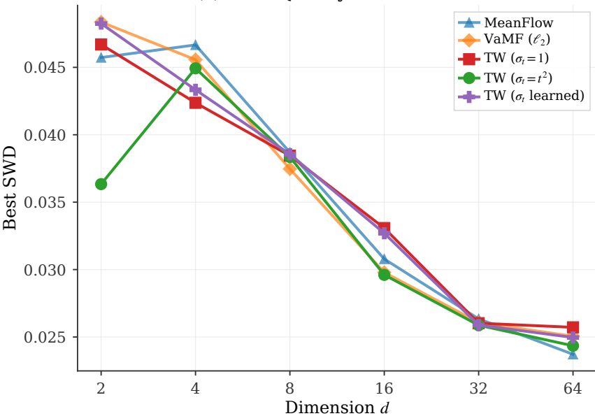
(a) Peak Quality vs Dimension
