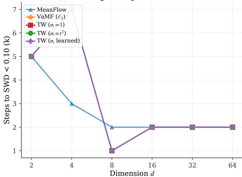
(b) Convergence Speed vs Dimension
