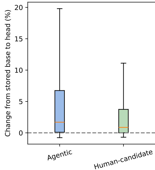
Mean file NLOC
