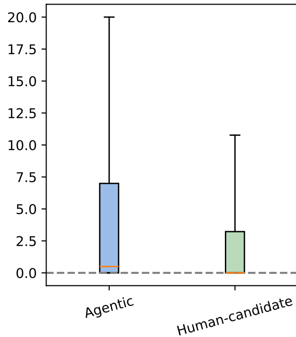
Mean file function count
