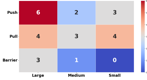
Figure 5: Push-pull-barrier heatmap.
