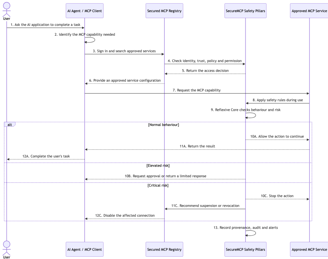
Numbered AI agent and LLM application journey
