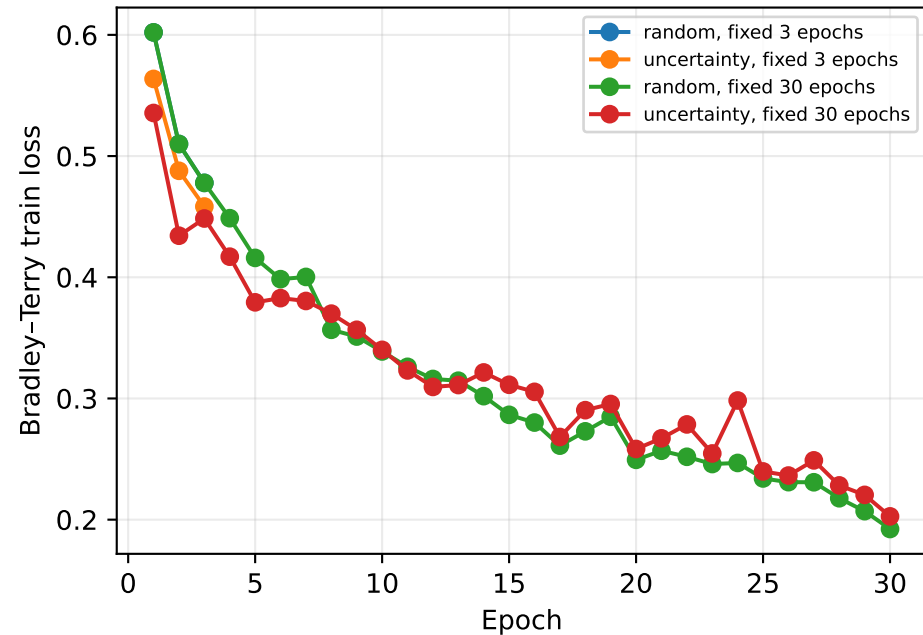
Budget 10: training dynamics
