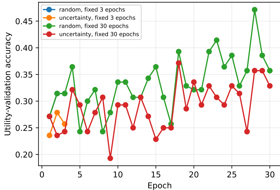
Budget 10: validation dynamics
