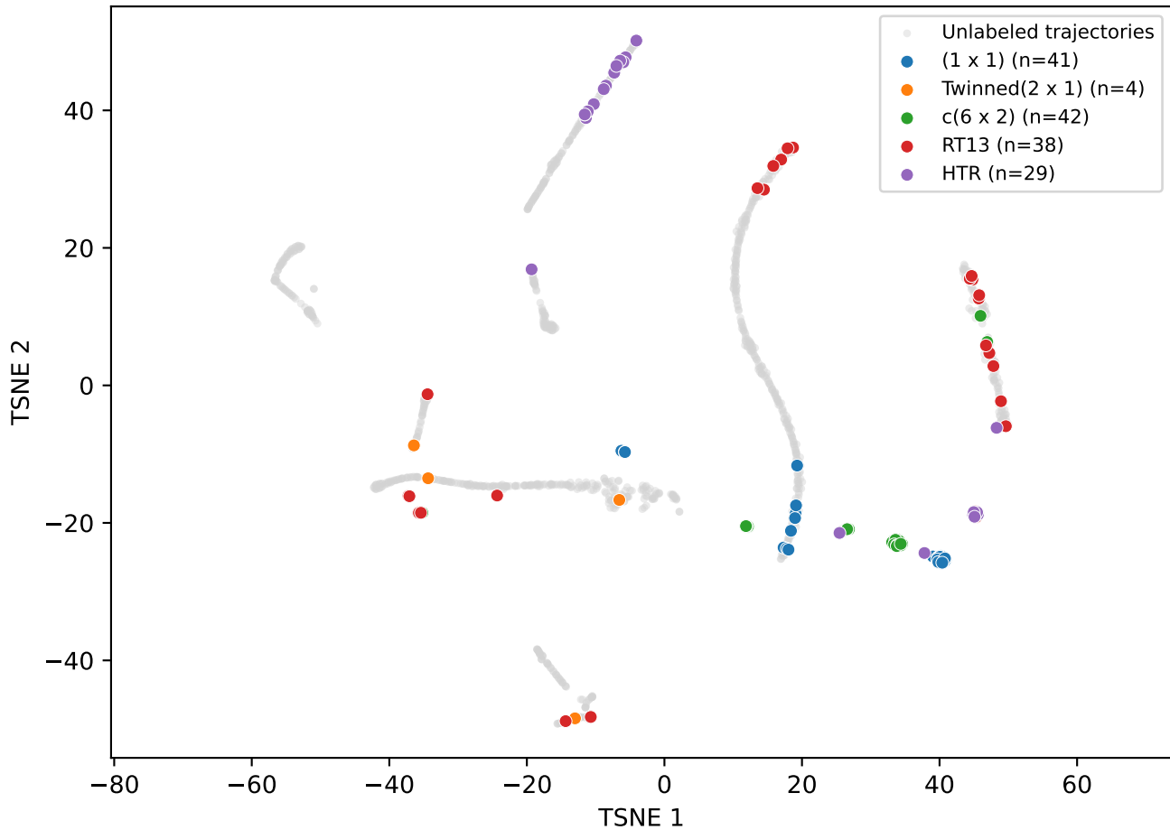
raw_pixels: TSNE fixed t-SNE protocol
