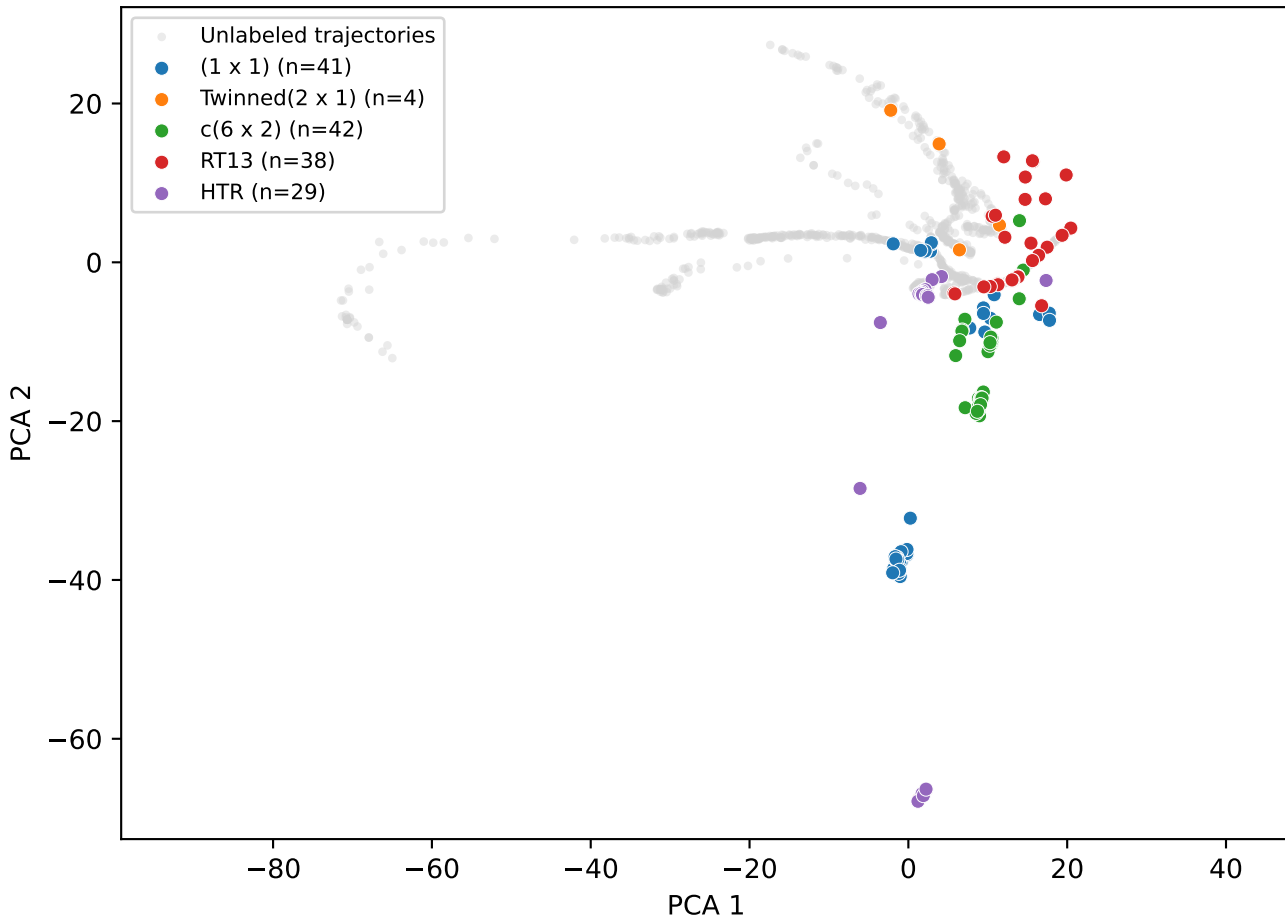
rhed_simclr_resnet18: PCA explained variance=0.762
