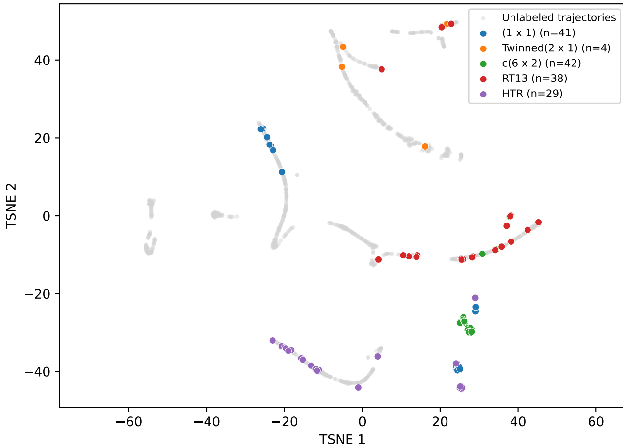
rheed_simclr_resnet18: TSNE fixed t-SNE protocol
