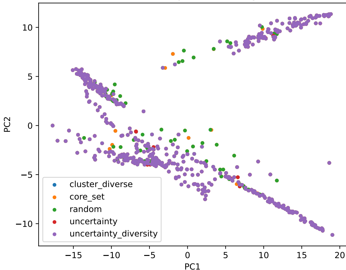
Stored selected pair embeddings: PCA
