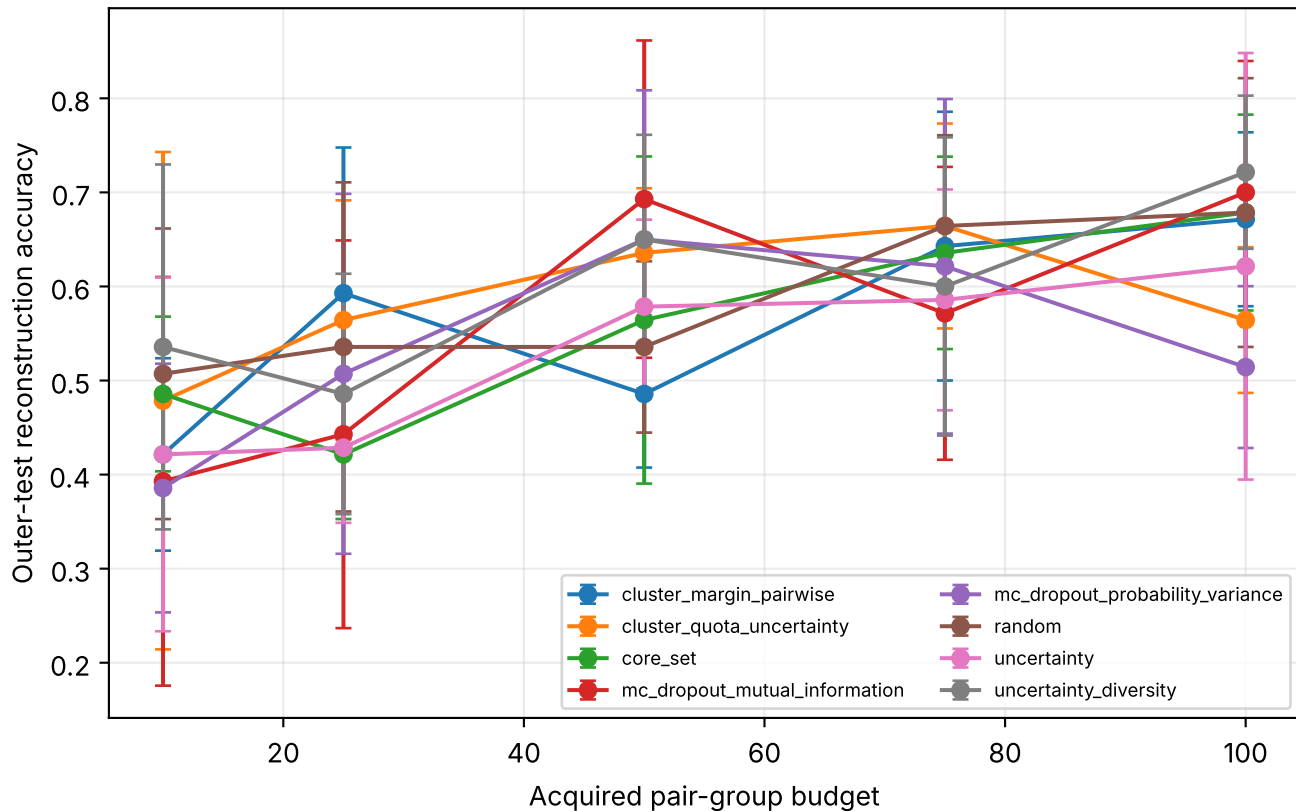
Identity-safe Task 3c | SimCLR | n=5 | validation-selected schedule
