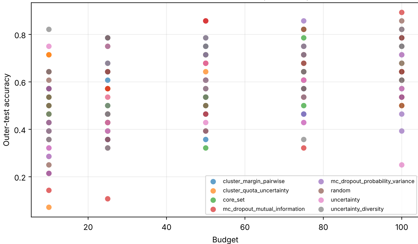
Seed-level outer-test outcomes | SimCLR | n=5
