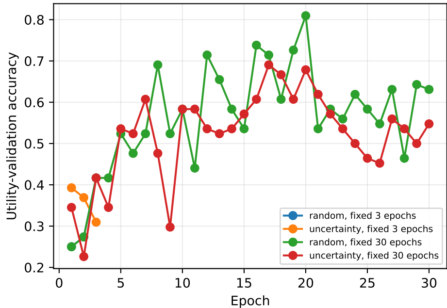
Budget 100: validation dynamics
