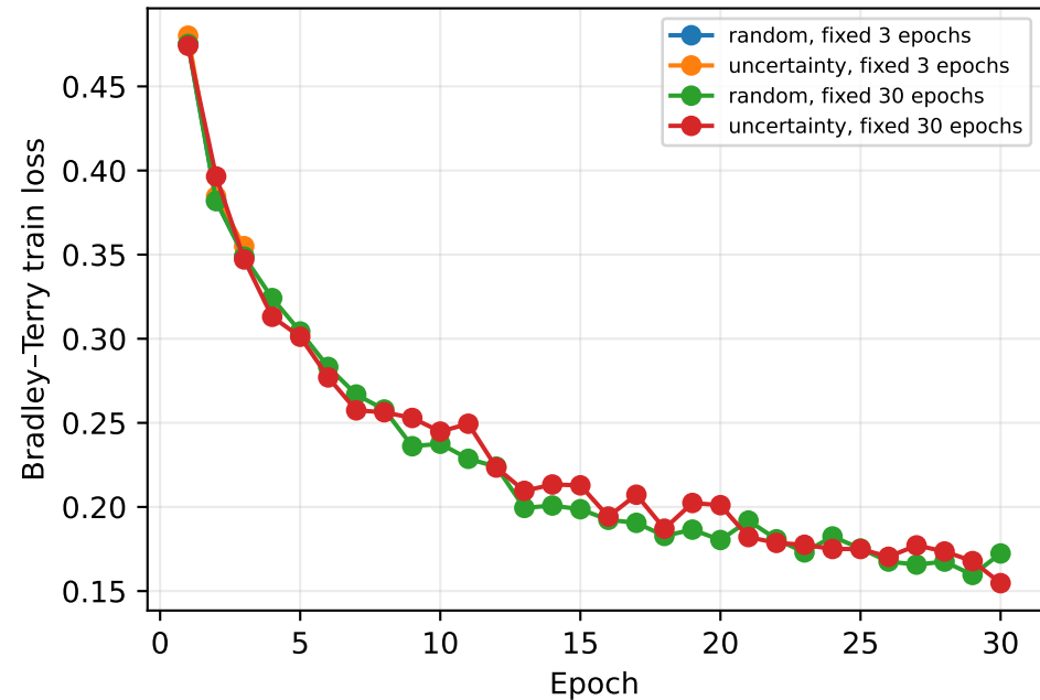
Budget 100: training dynamics
