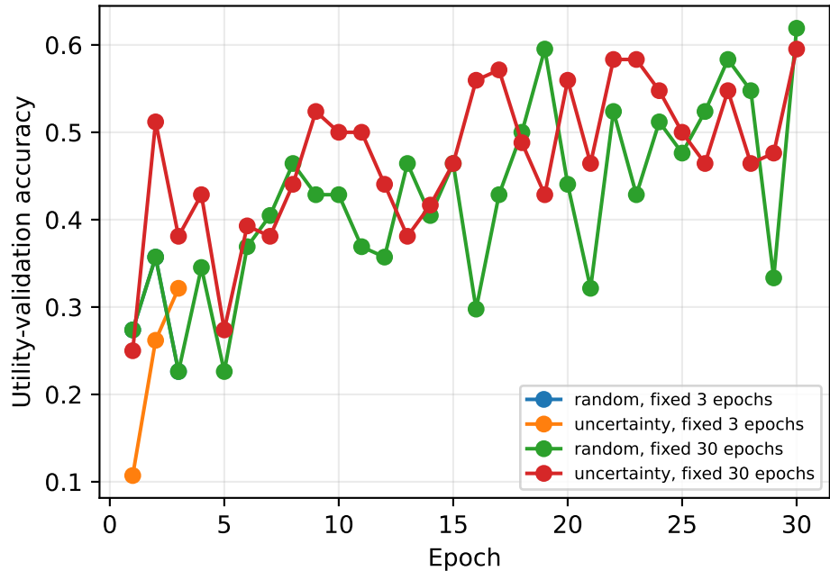
Budget 25: validation dynamics
