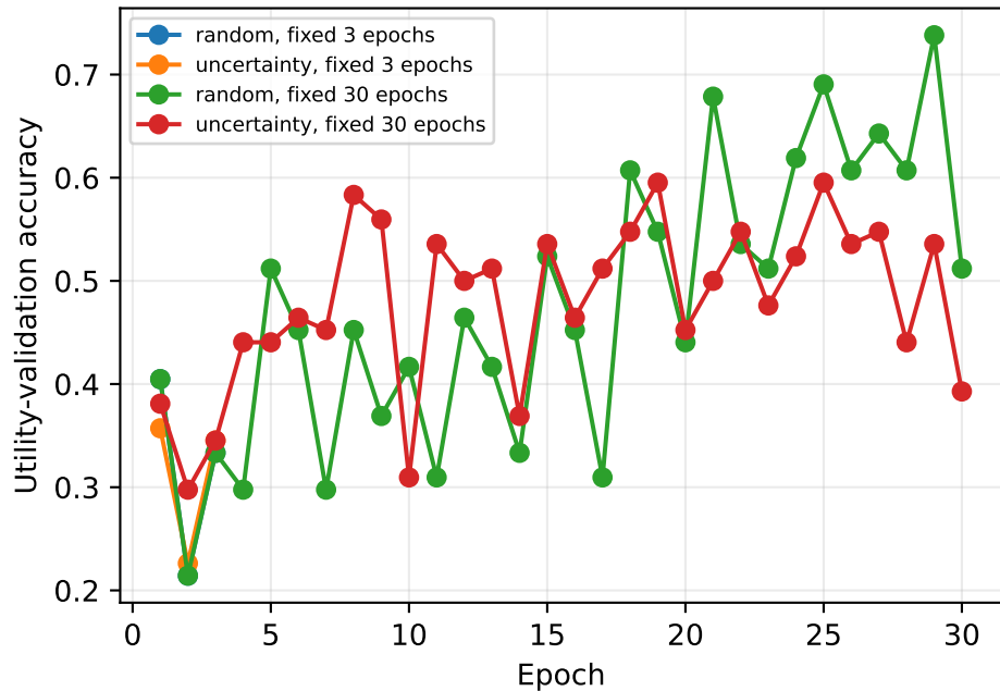
Budget 75: validation dynamics
