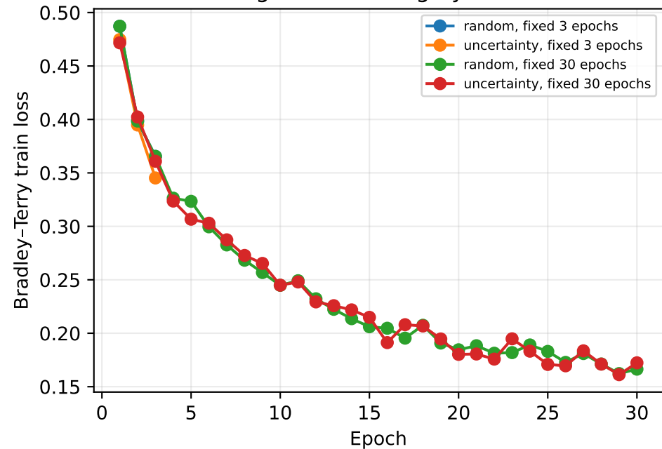
Budget 75: training dynamics
