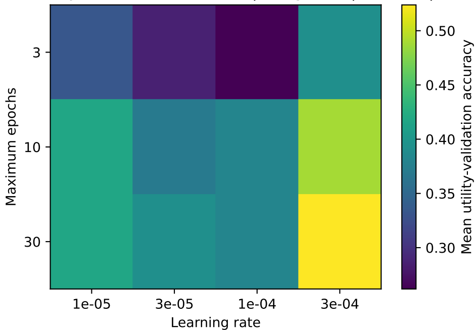
Validation-only schedule calibration | budget 10 | SimCLR | n=3
