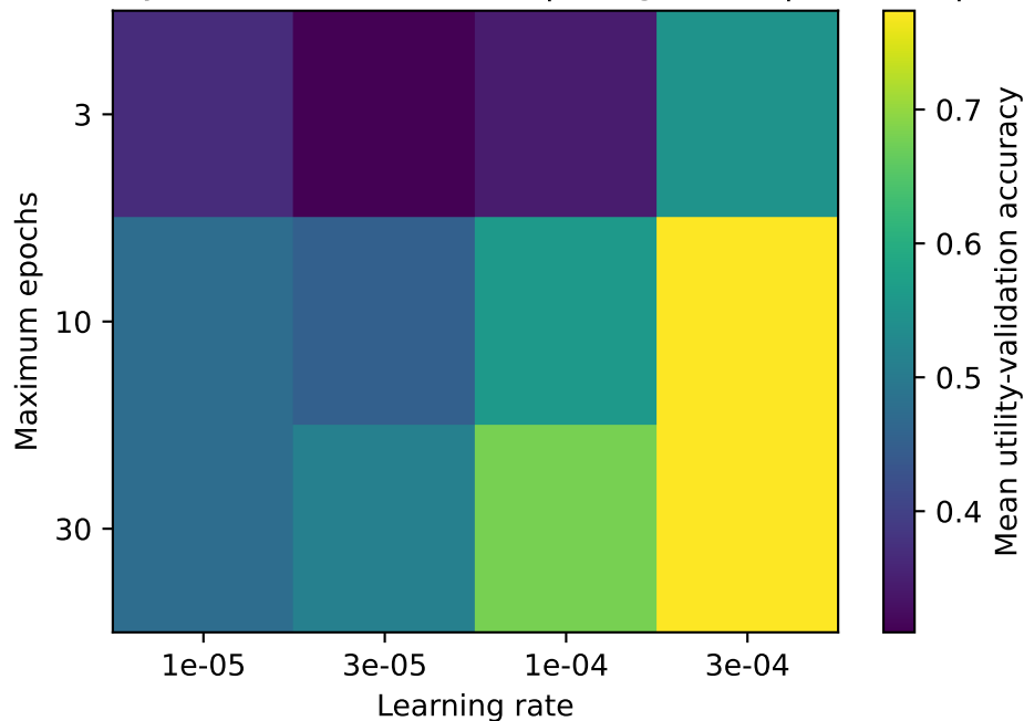
Validation-only schedule calibration | budget 100 | SimCLR | n=3
