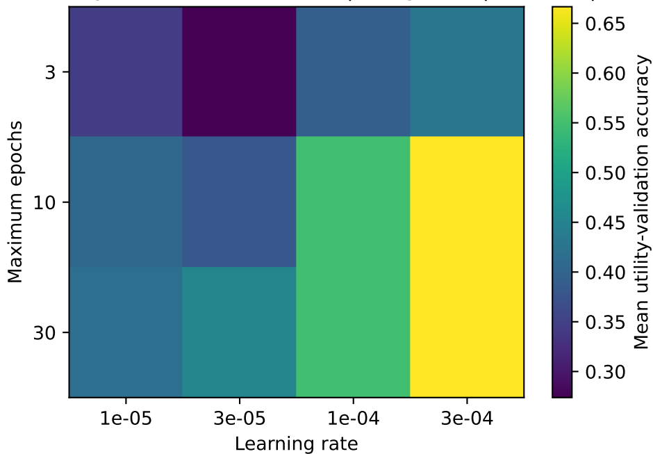
Validation-only schedule calibration | budget 25 | SimCLR | n=3
