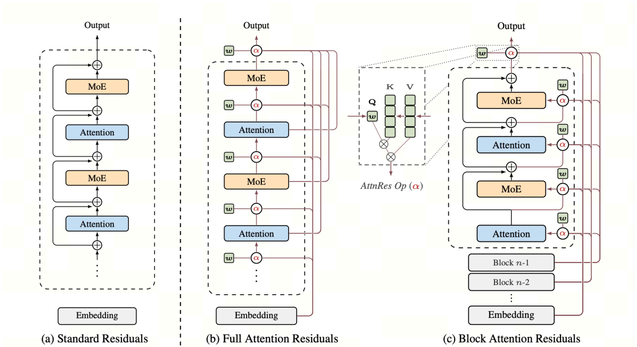
Figure 1: Overview of Attention Residuals. (a) Standard Residuals: standard residual connections with uniform additive accumulation. (b) Full AttnRes: each layer selectively aggregates all previous layer outputs via learned attention weights. (c) Block AttnRes: layers are grouped into blocks, reducing memory from O(Ld) to O(Nd) .
