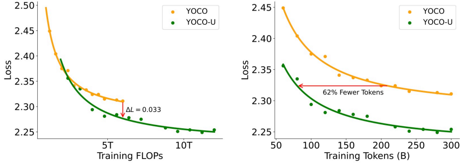
Figure 2: Scaling behavior of language modeling loss with the same model size. (Left) Loss versus training FLOPs: YOCO-U achieves competitive or lower loss ( \Delta L=0.033 ) at the same FLOPs budget, while incurring negligible KV cache overhead. (Right) Loss versus training tokens: YOCO-U also improves data efficiency, requiring approximately 62% fewer tokens to reach comparable performance.
