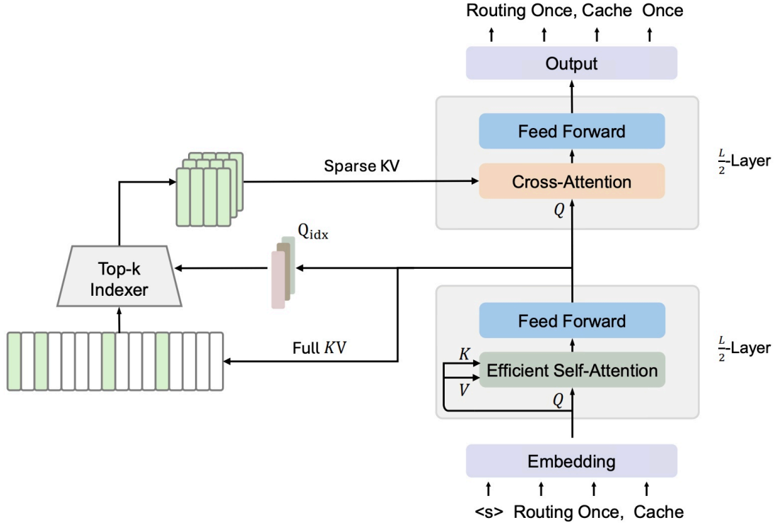
Figure 1: Overview of cross-layer sparse attention. The self-decoder first produces a shared KV cache, which is computed only once and then reused by all subsequent cross-decoder layers. During this stage, a shared query-aware indexer jointly generates the routing queries and keys and computes a token-level sparse top- k index for each query token. This sparse index is also produced only once and is shared across the following cross-decoder layers, allowing them to reuse the same selected KV positions instead of recomputing layer-specific sparse routing.
