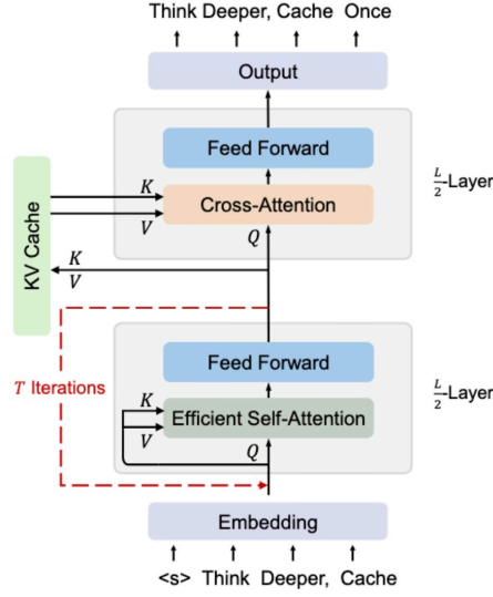
Figure 1: Overview of the YOCO-U architecture. Universal Self-Decoder (bottom) performs recursive computation ( T iterations, indicated by the red dashed line) using efficient self-attention (local windows) to refine representations. Crucially, the global KV cache produced for cross-attention is generated once and remains constant regardless of T , while only the local window-based KV caches grow with iterations, keeping overall cache overhead negligible. Cross-Decoder (top) reuses this shared global KV cache via cross-attention for autoregressive token prediction.
