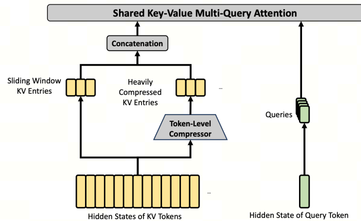
Figure 4 | Core architectures of HCA. It performs heavier compression, where the KV entries of m' ( \gg m ) tokens will be consolidated into one. Also, we additionally introduce a small set of sliding window KV entries to enhance local fine-grained dependencies.
