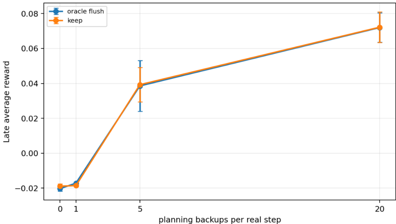
Late average reward by planning budget and model handling in the 20-seed extended run.
