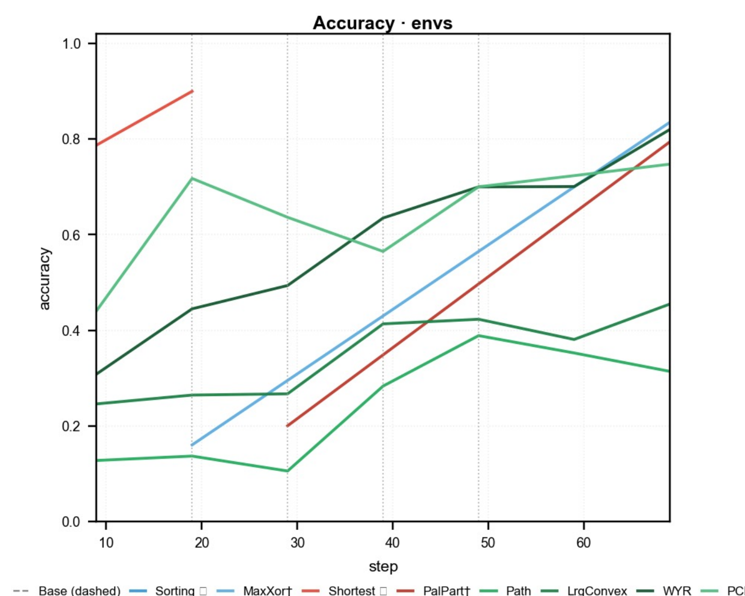
Fig 2. Comparison of training accuracy of 8 envs
