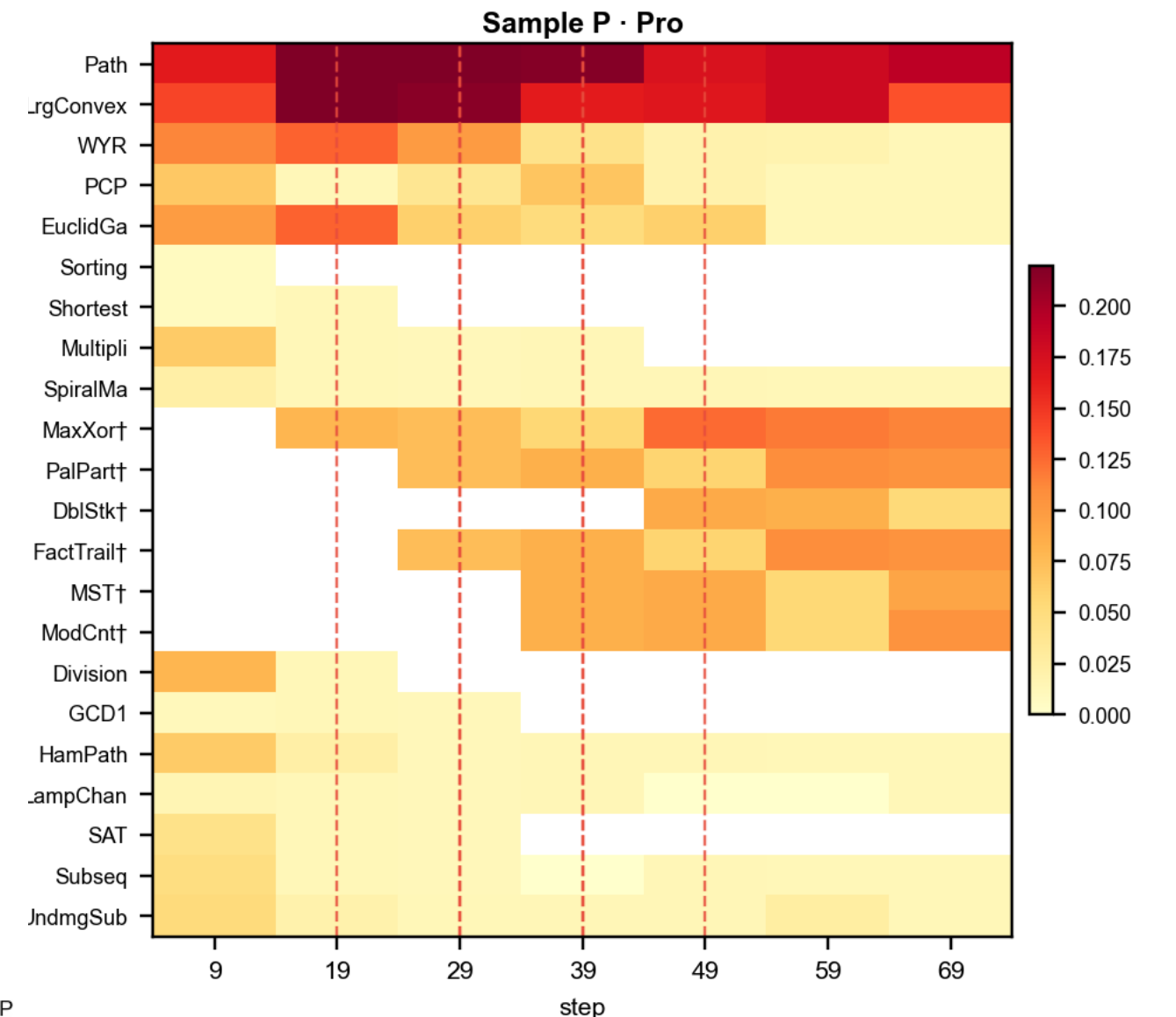
Fig 3. Comparison of sampling rate versus steps
