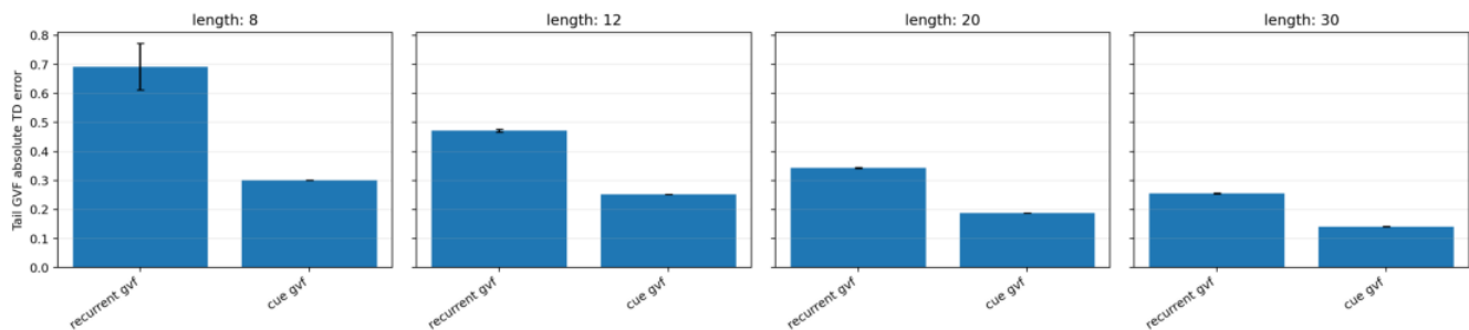
Tail GVF absolute TD error for GVF-based state constructions.
