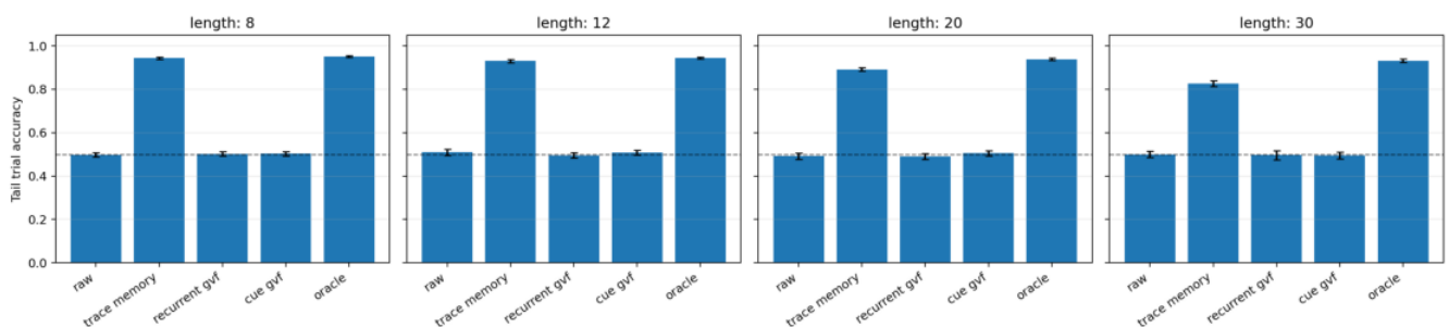
Tail trial accuracy by state construction and maze length.
