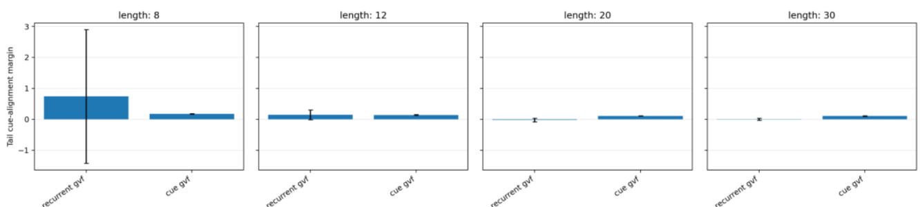
Tail cue-alignment margin for GVF-based state constructions.
