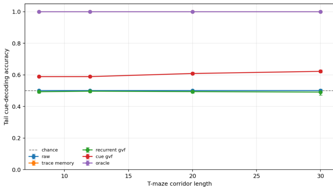
Tail cue-decoding accuracy by state construction and maze length.
