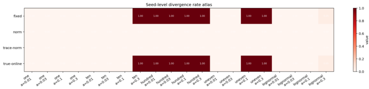
Seed-level divergence-rate atlas by algorithm, scale, and alpha.
