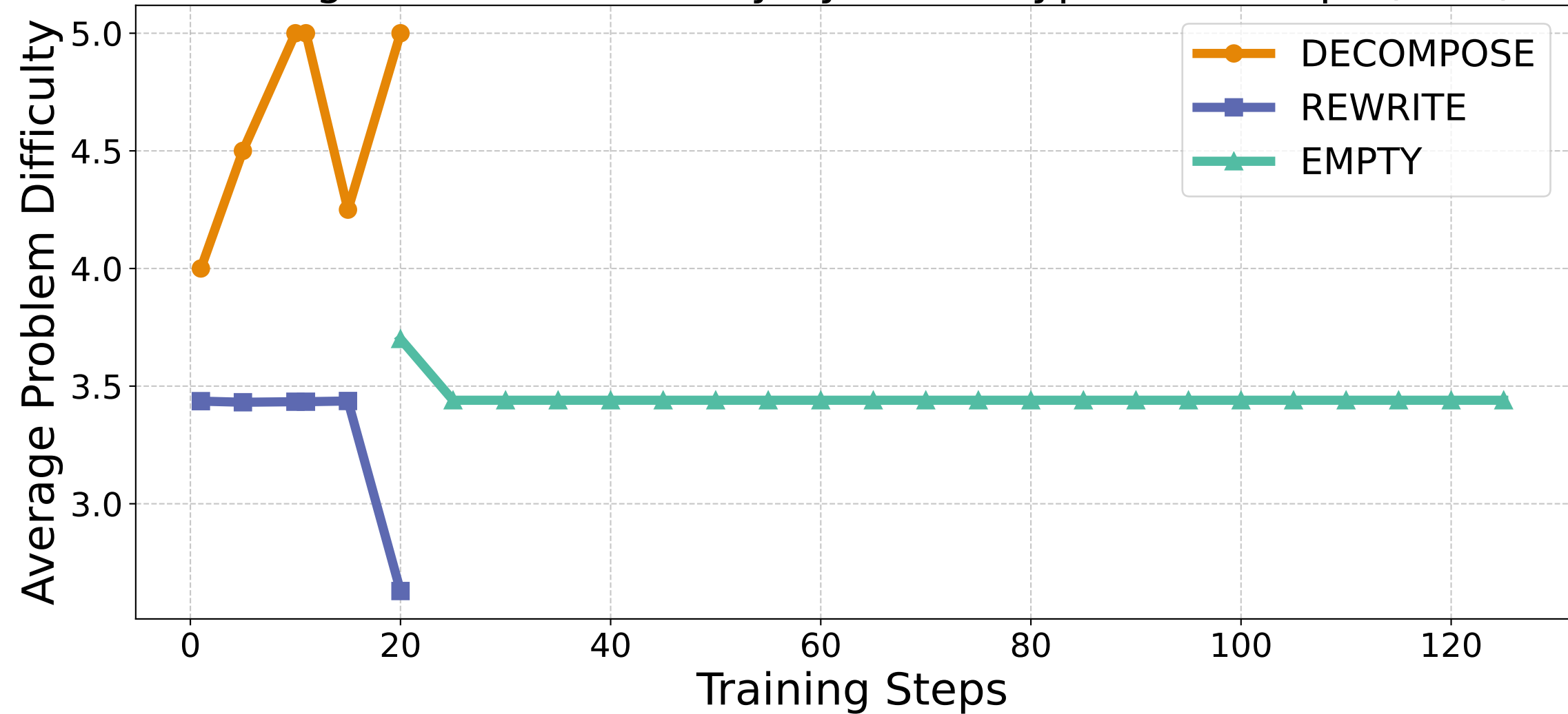
Average Problem Difficulty by Action Type Over Steps (h1l1)
