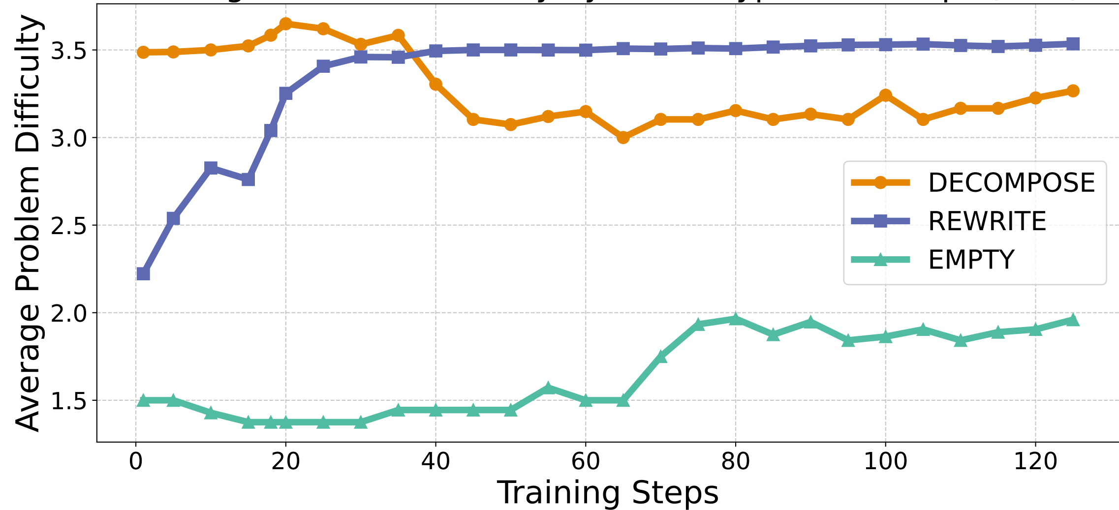
Average Problem Difficulty by Action Type Over Steps (h8l8)
