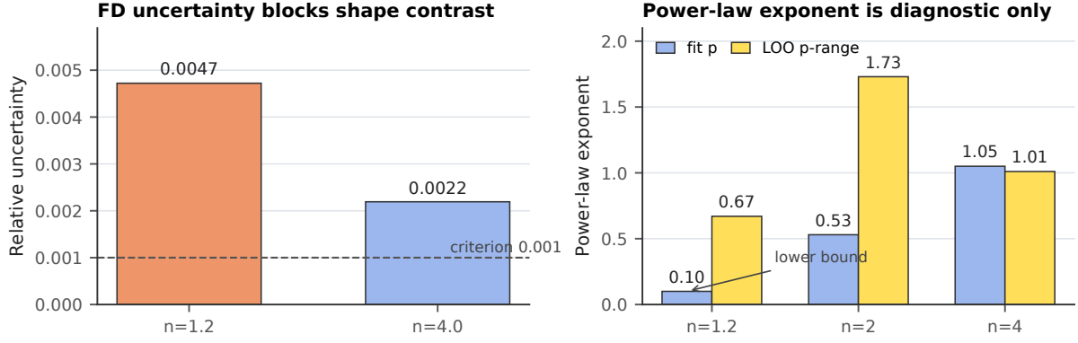
FIG. 3. Continuum-reference and TB-only scaling diagnostics from existing outputs. The FD reference uncertainties for non-circular shapes exceed the 10^{-3} criterion used before shape-sensitive residual analysis. The TB-only power-law exponents are accompanied by large leave-one-size-out ranges and are not treated as physical exponents.
