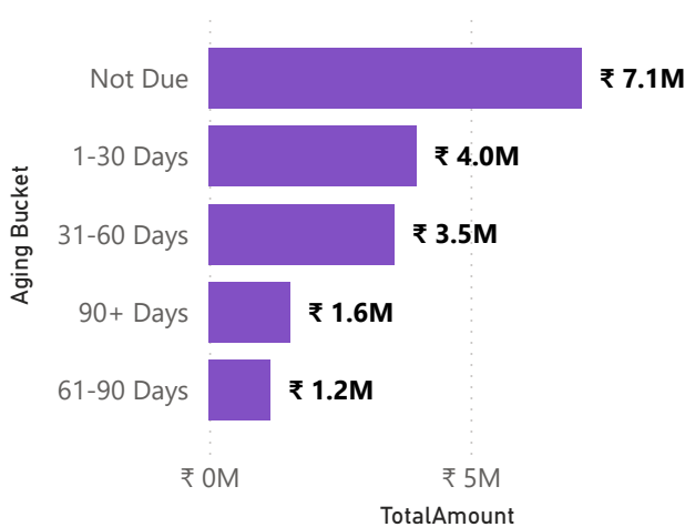
Aging analysis
