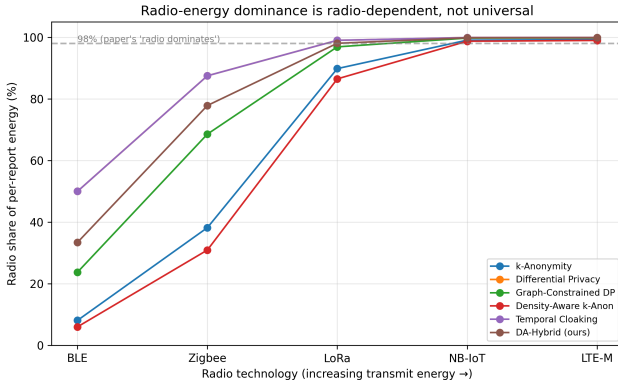
Fig. 7. Radio share of per-report energy vs. radio technology. Radio dominance is radio-dependent, not universal.
