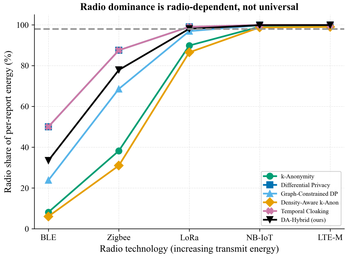
Figure 10: Radio share of per-report energy vs. radio technology. Radio dominance is radio-dependent, not universal.
