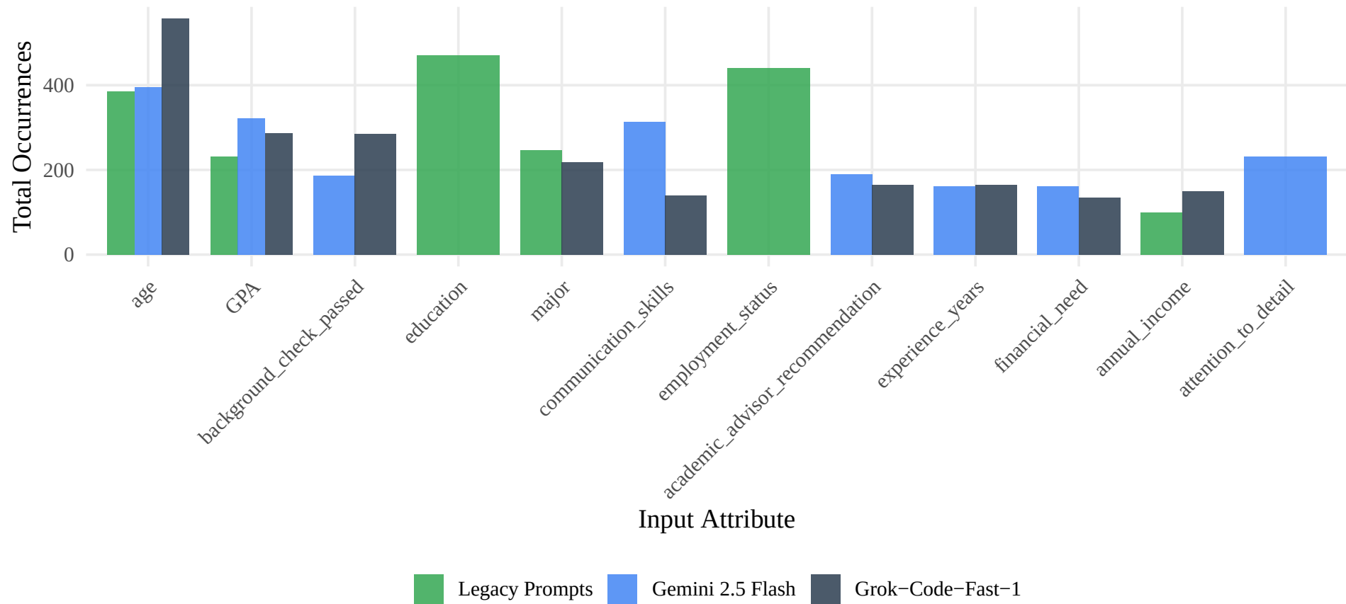
Top 12 Most Frequently Utilized Attributes Across Models
