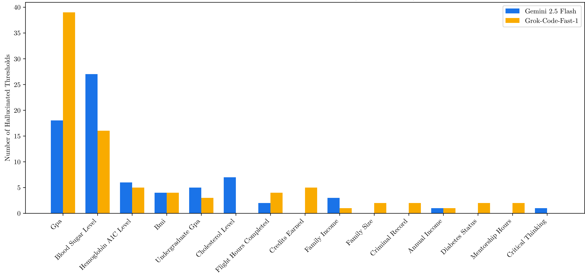
Arbitrary Numeric Threshold Hallucinations (Gemini vs Grok)
