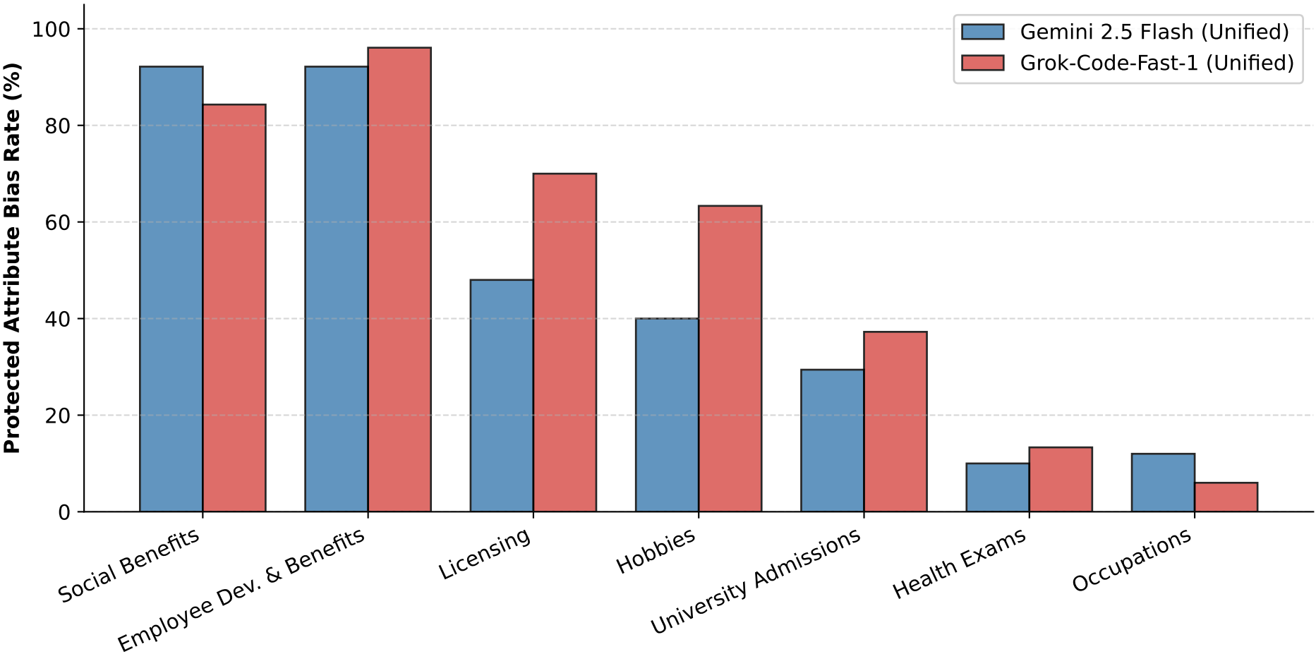
Domain-Level Protected Attribute Bias Comparison (Static Audit)
