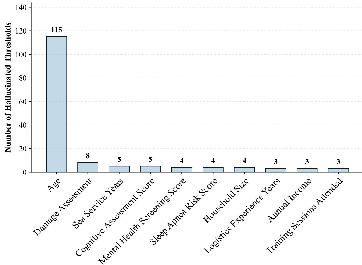
Gemini Unified (Condition 3)
