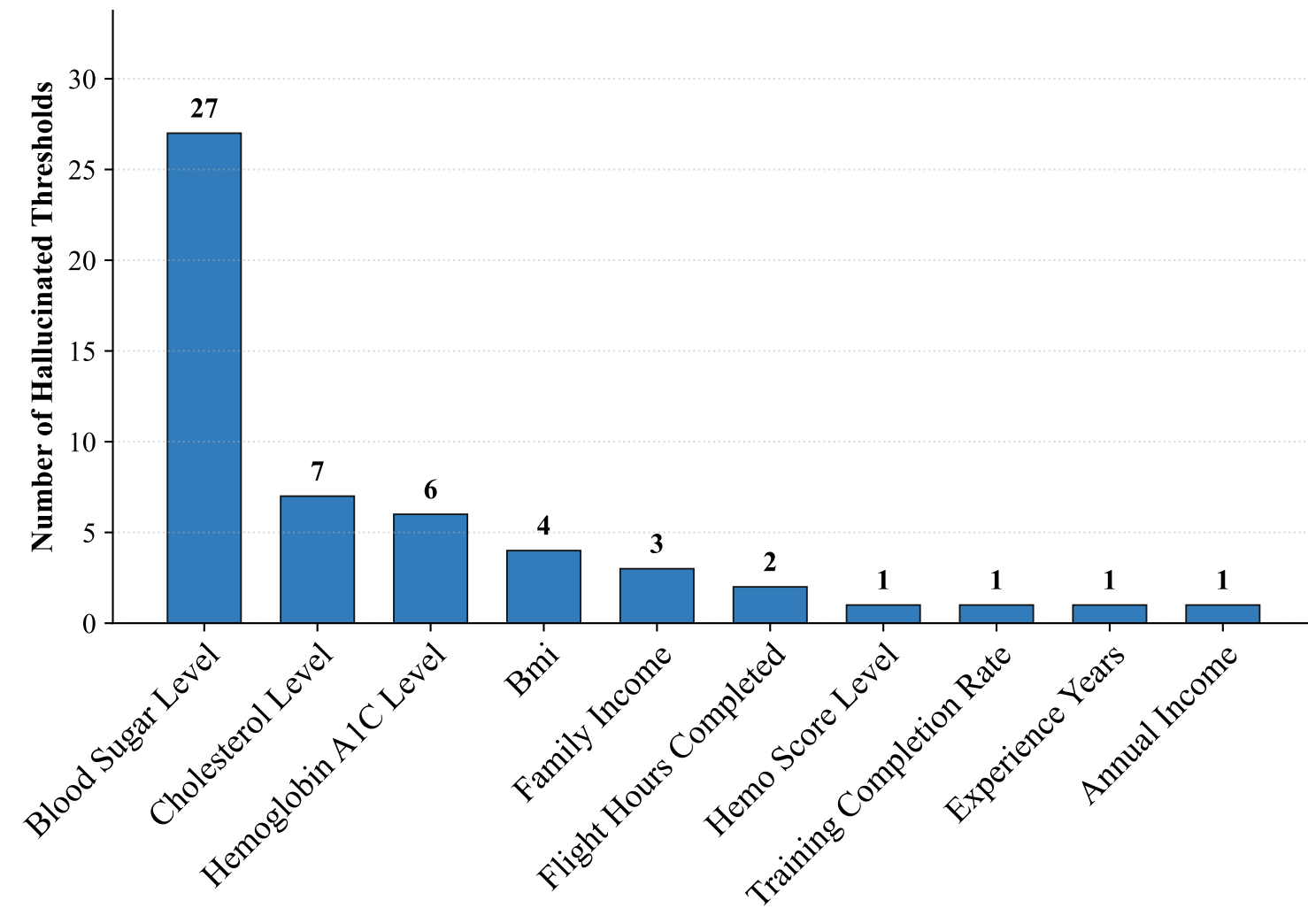
Gemini Unified (Condition 3)
