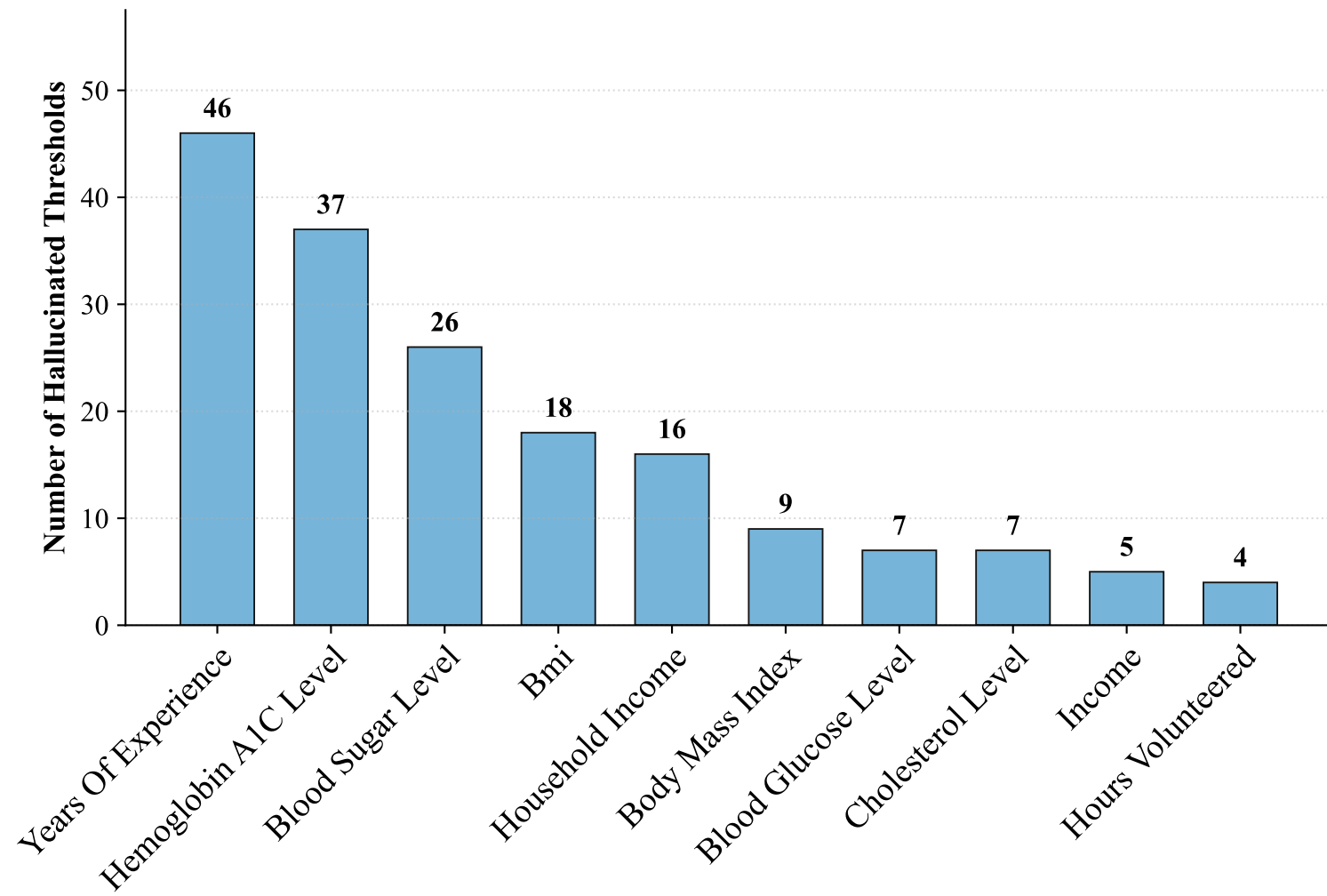
Gemini Expanded (Condition 2)
