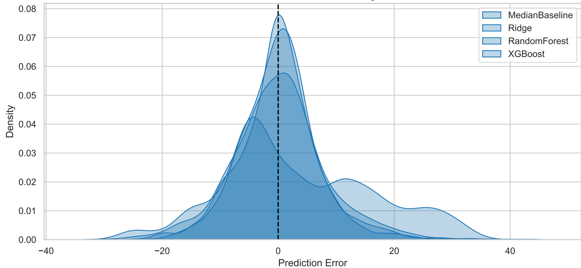
Prediction Error Distribution – Regime A
