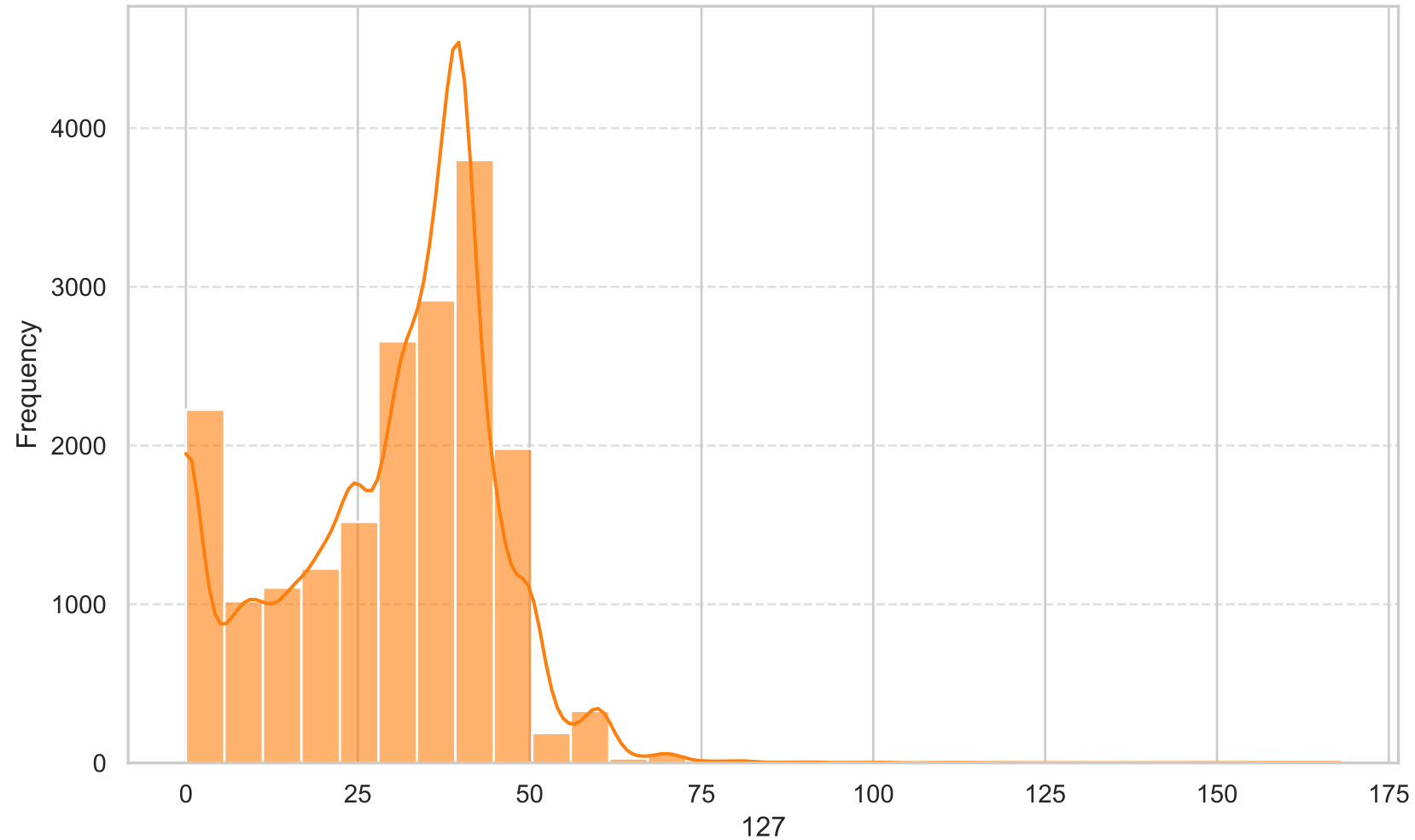
Distribution of 127 – Regime B (2014–2019)
