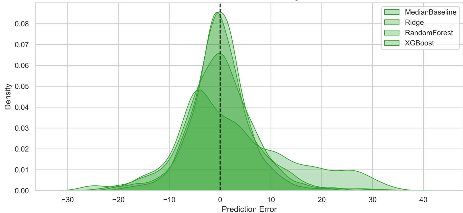
Prediction Error Distribution – Regime C
