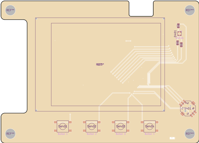
Top Assembly (Scale 1:1)
