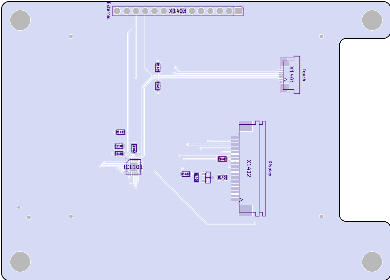
Bottom Assembly (Scale 1:1)
