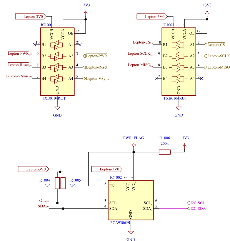
Level shifting (Lepton IO <math>\leftrightarrow</math> System Voltage)
