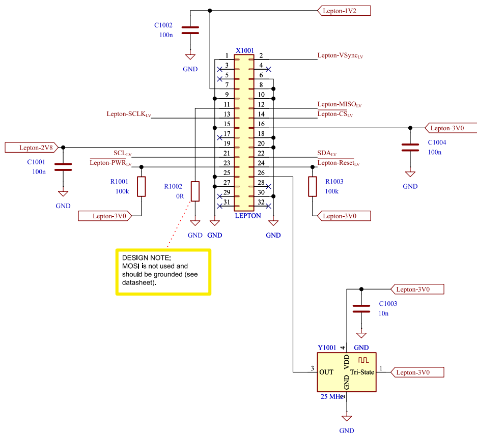
Lepton 3.5 camera connector
