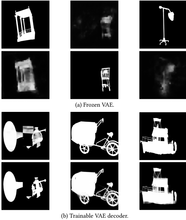
Figure 3: Qualitative comparison of two VAE training variants in the modified model. The frozen VAE variant produces diffuse foreground blobs, while training the VAE decoder improves object sharpness and boundary recovery.
