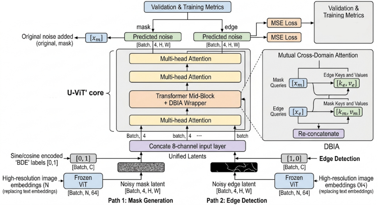
Figure 1: Architecture of the modified DiffDIS model. The original U-Net denoiser is replaced with a UniDiffuser-style transformer core, while ViT image embeddings, BDE labels, mask/edge latent paths, and mutual cross-domain attention provide task conditioning and mask-edge interaction.
