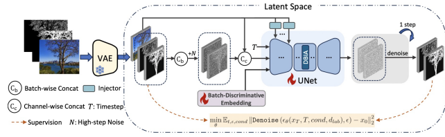
Figure 2: Original DiffDIS pipeline from the project assets. Our modification keeps the latent mask/edge formulation and one-step denoising objective, but replaces the U-Net denoising backbone with a UniDiffuser transformer and adds ViT-based image conditioning.
