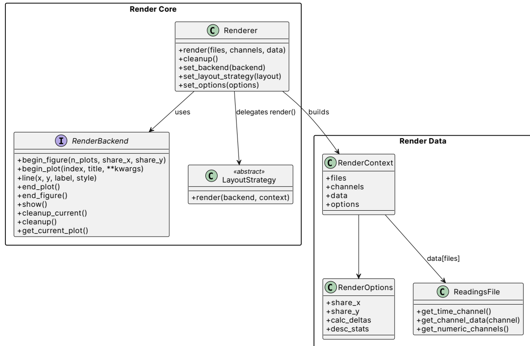
Figure 4. 3: Architecture of the rendering system, showing the core components and their interactions
