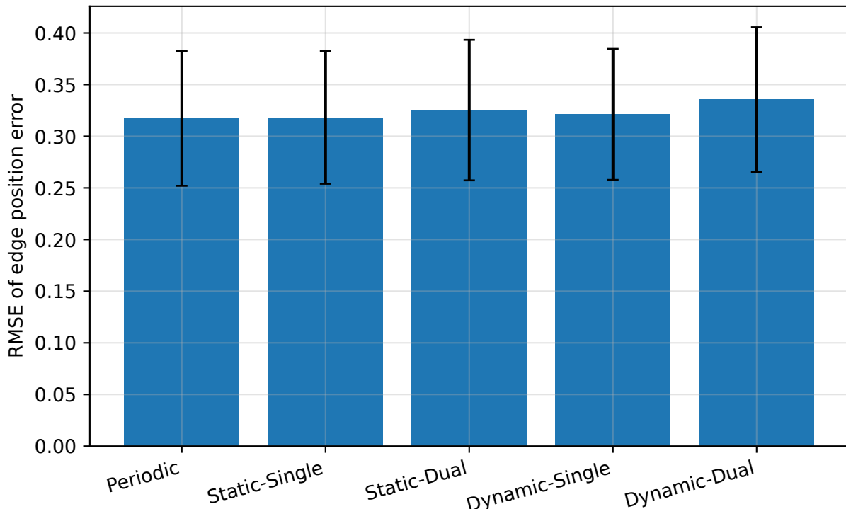
Window RMSE (mean \pm std over 10 seeds)
