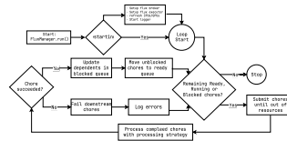
Figure 3: Manager Loop
