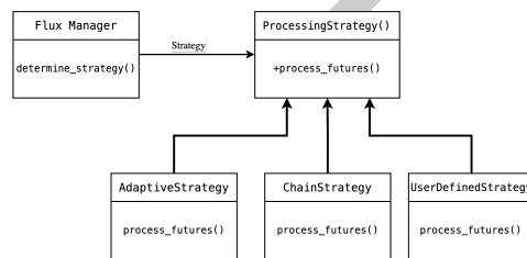
Figure 4: Strategy Pattern
