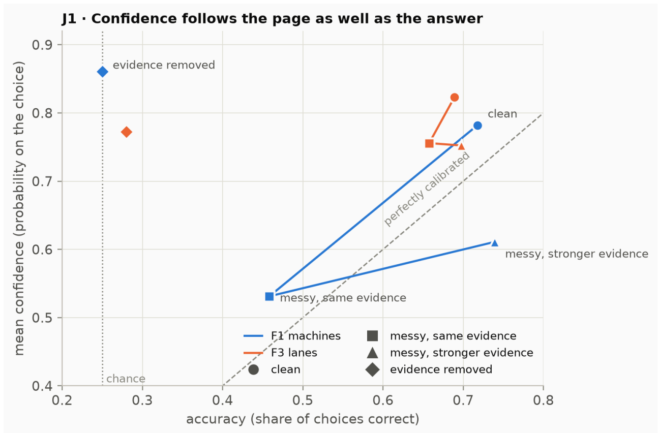
Figure 2. Confidence follows the page as well as the answer. Mean confidence against accuracy for each arm. On the dashed line, confidence equals accuracy. In F1, moving from the clean to the reworked layout at the same evidence lowers confidence along with accuracy, the pattern of a system that knows its own reliability. Restoring accuracy with stronger evidence leaves confidence low, which exposes the fall as a reading of the layout. With evidence removed, confidence stays high at chance accuracy.
