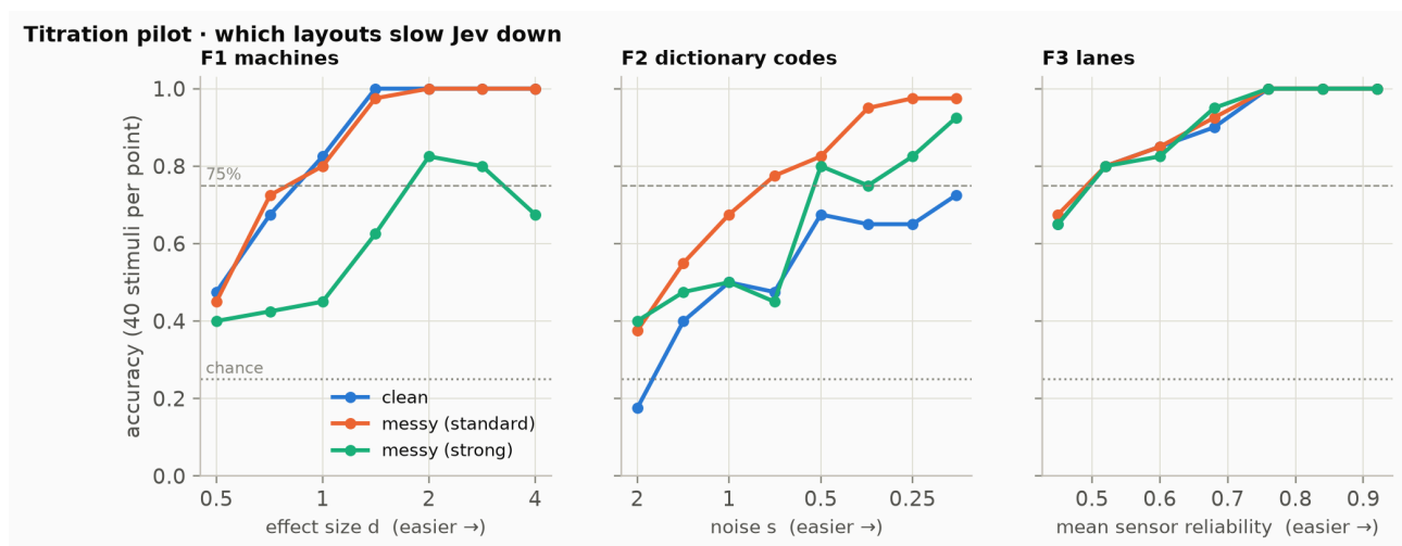
Figure 1. Which layouts slow Jev down. Accuracy by difficulty in the pilot, 40 stimuli per point, one call each. F1: the standard reworked layout costs nothing; converting some readings to per-minute units costs a great deal. F2: Jev never exceeds 0.73 on the clean wide table and falls below chance at the hardest level, yet the “reworked” list layout is easier for it (0.97). F3: no layout slows it.
