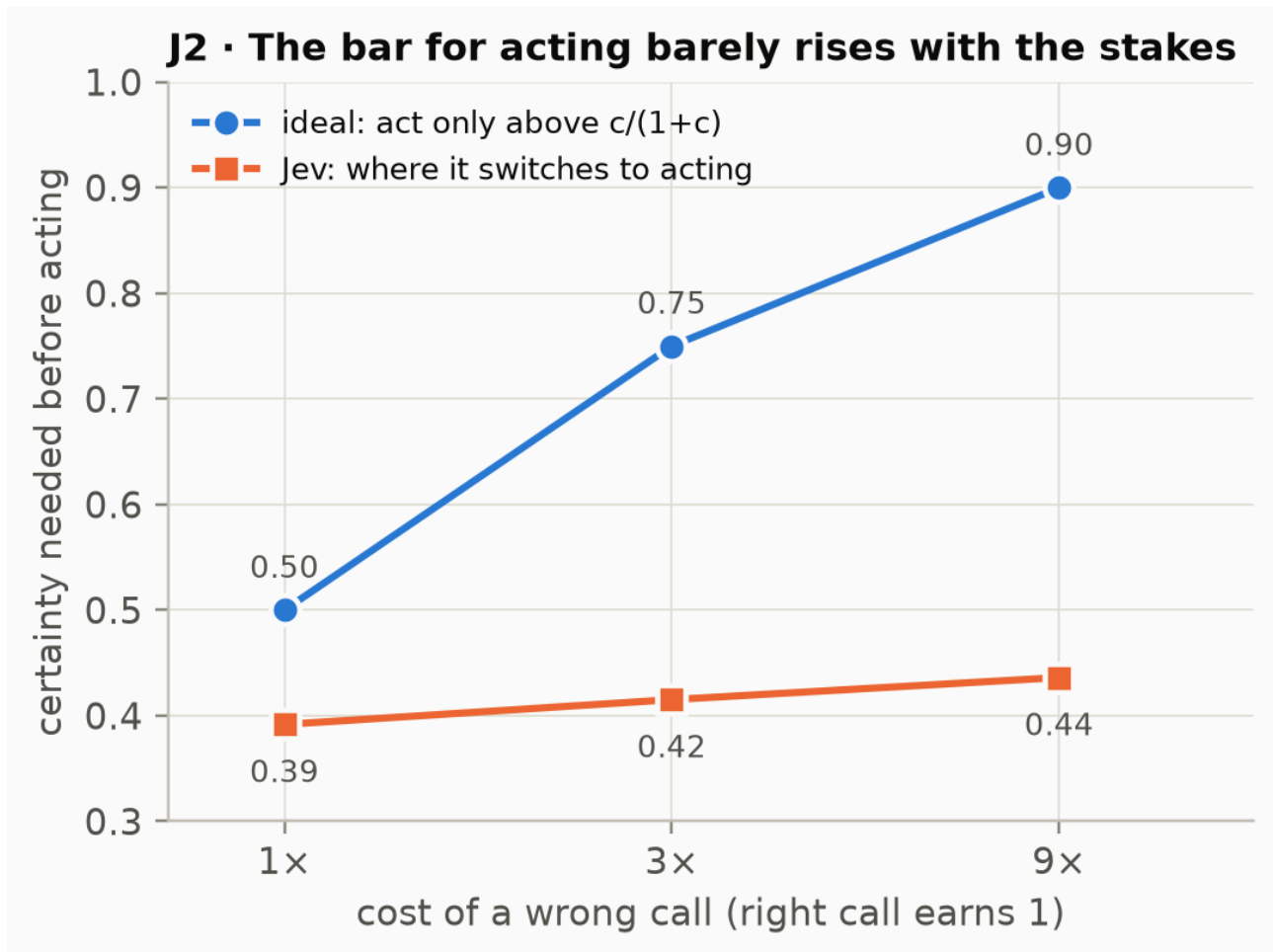
Figure 4. The bar for acting barely rises with the stakes. The certainty needed before acting: ideal ( c/(1 + c) ) against Jev's fitted switch point, the probability of being right at which its probability of holding crosses 0.5.
