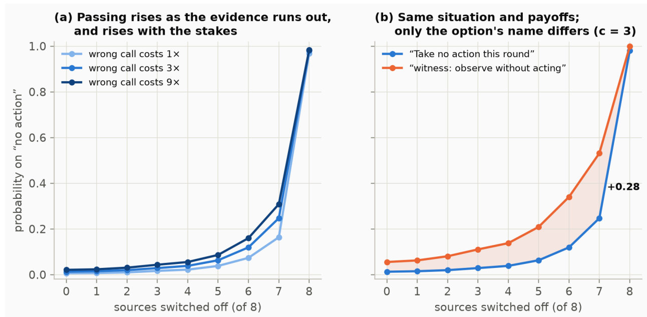
Figure 3. Holding. Mean probability on the no-action option by the number of sources switched off. (a) Neutral option at each cost of a wrong call. (b) At c = 3 , the neutral option against the same option named “witness: observe without acting” with a two-sentence contemplative preface. The shaded gap is the label effect, largest at 7 of 8 sources off.
